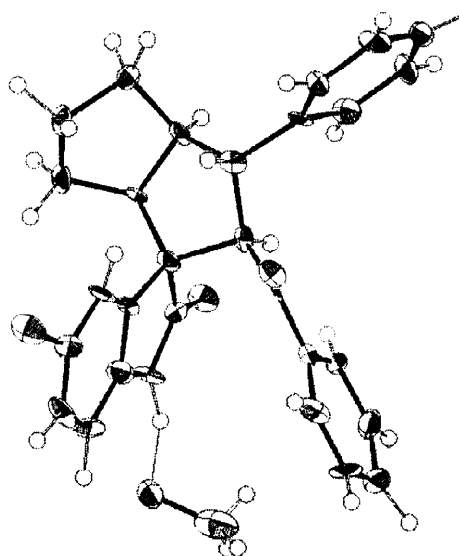
Single crystal X-ray structure of a spiro[pyrrolidine-2,3'-oxindole]. Unit cell contains one methanol of crystallization (ORTEP representation)
