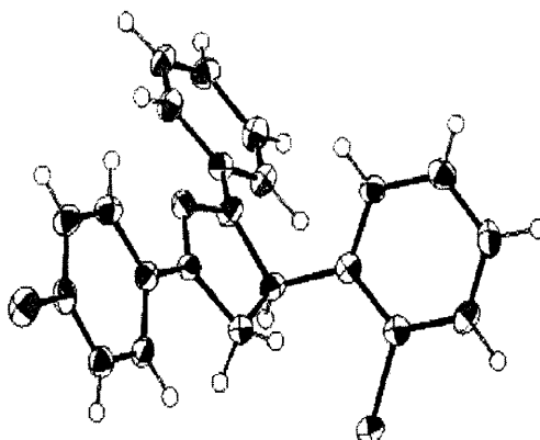
Single crystal X-ray structure of N-phenyl-3-(4-fluorophenyl)-5-(2-chlorophenyl)-pyrazoline (ORTEP representation)
